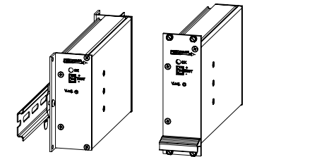
DIN-rail mounted Model with N + TS35 clips 19" subrack mounting Model with L-panel (opt.)
