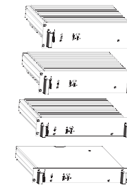
PSC600-series for 19" subrack mounting, Model with L-panel 10TE, 12TE and 14TE (optional)
