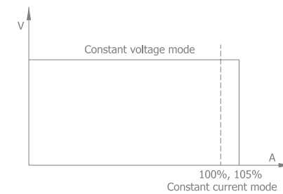
Rectangular current limit characteristic of Polyamp DC/DC converters
