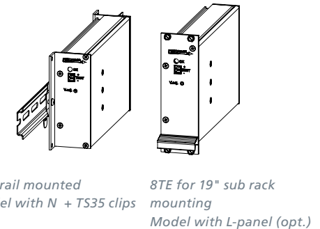
DIN or wall mounting Model with N (standard)
