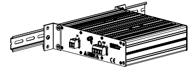
PM500 R DIN- or wall-mounted, brackets L58-1 + TS35 clips Option 400065
