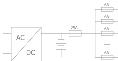
This figure shows a traditional battery charging system with a battery and battery fuse. After that is the downstream fuse distribution.
