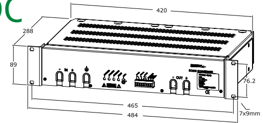
PC1000/2000 Rackmounted 19" 2U. Brackets L89-3 (std)
