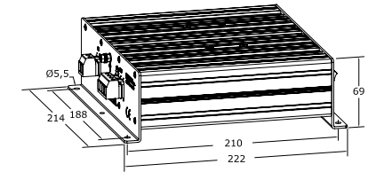
PM250/500 Standard for wall- or DIN mounting
